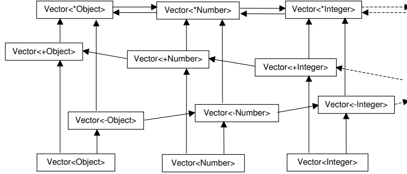
Fig. 1. Subtyping graph of variant parametric types
